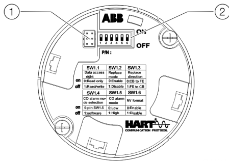
Figure 2: HART communication board / 4 to 20 mA
