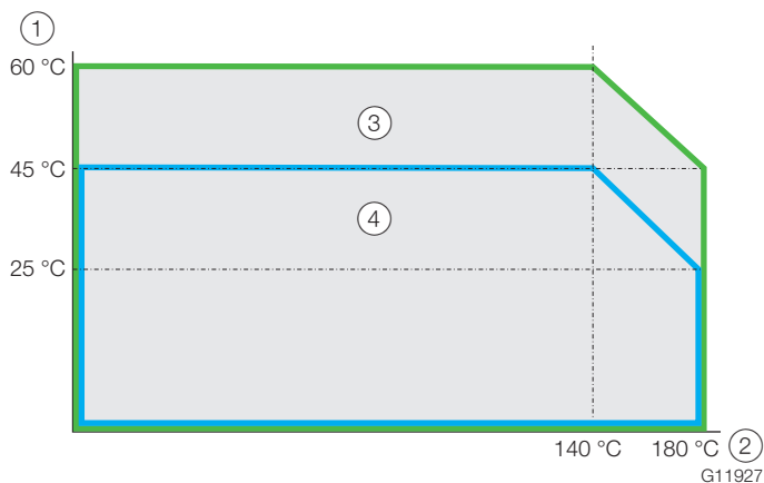
Fig. 3: High temperature design
