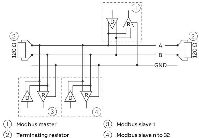
Figure 1: Communication via Modbus protocol
