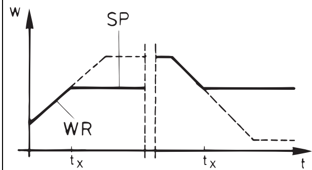
Change of ramp setpoint
