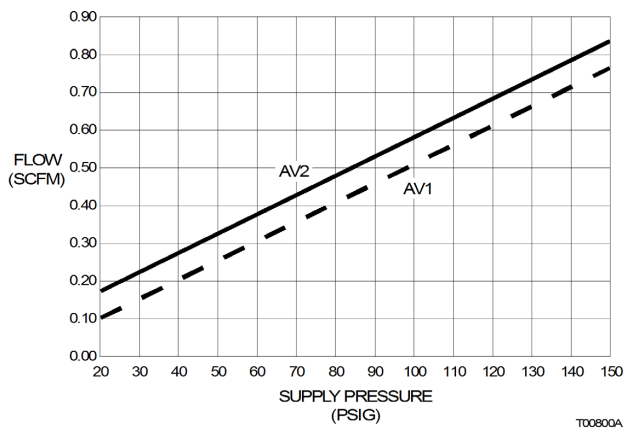
Figure 1-2. Air Consumption
