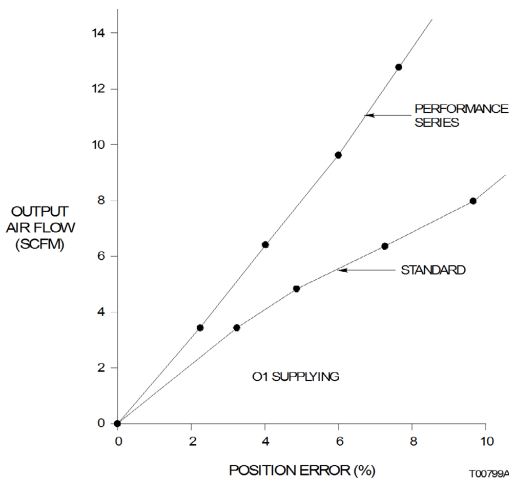
Figure 1-4. Expanded First Quadrant View of Figure 1-3
