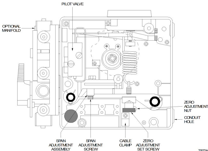
Figure B-12. Calibration Adjustments
