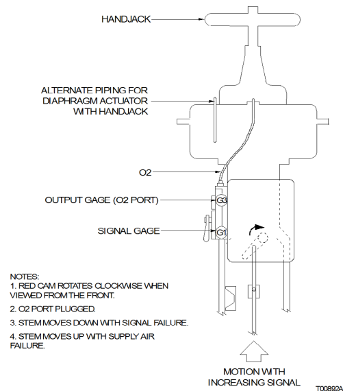
Figure B-7. Reverse Acting, Top Loaded, Single Acting Tubing Example
