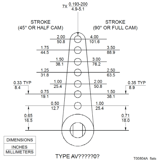
Figure B-3. Drive Arm Connections
