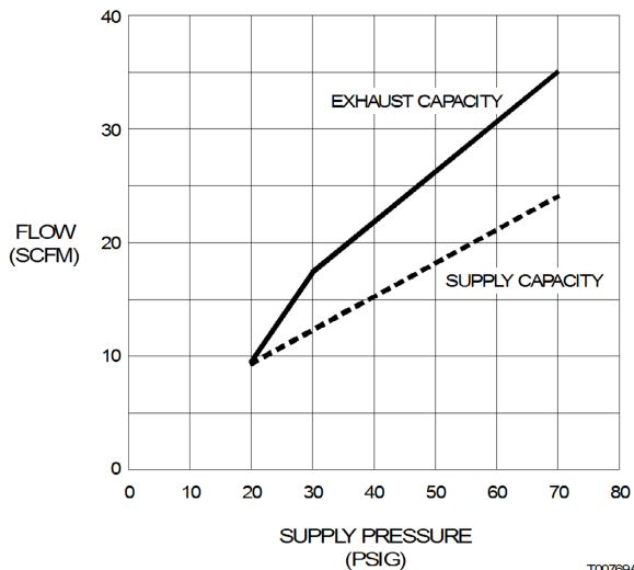
Figure 1-1. Capacity (Exhaust to Atmosphere)
