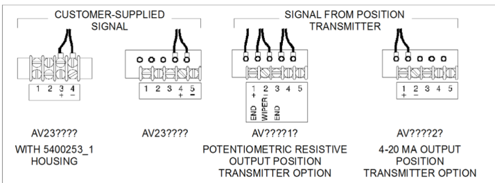
Figure B-11A. Electrical Connections
