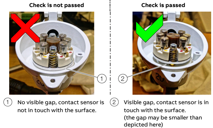
Figure 4: BUZ housing
