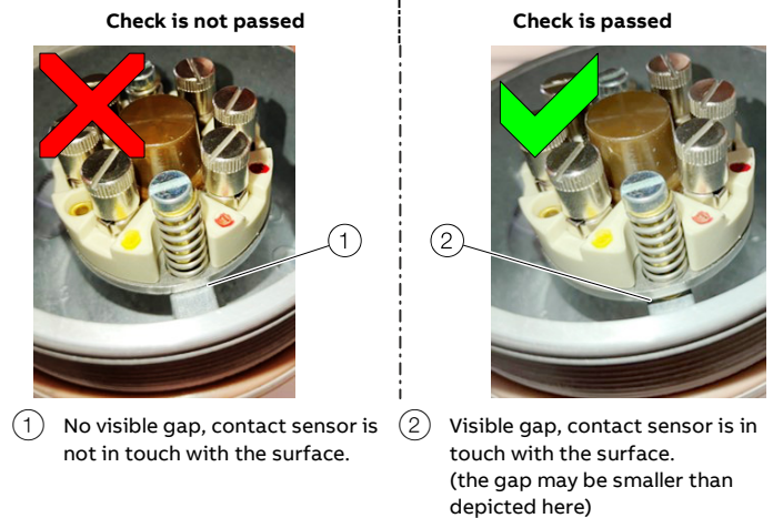
Figure 5: AGL/AGS housing
