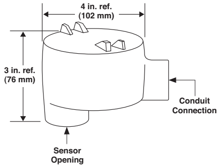
Approximate Assembled Dimensions: 4 in. H x 2 1/4 in. L x 3 in. W
