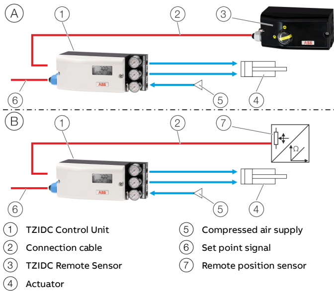
Figure 6: TZIDC with external position sensors
