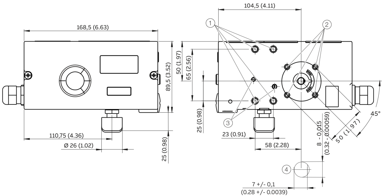
Figure 15: Top view
