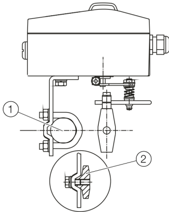
Figure 2: Mounting on linear actuators in accordance with DIN / IEC 534
