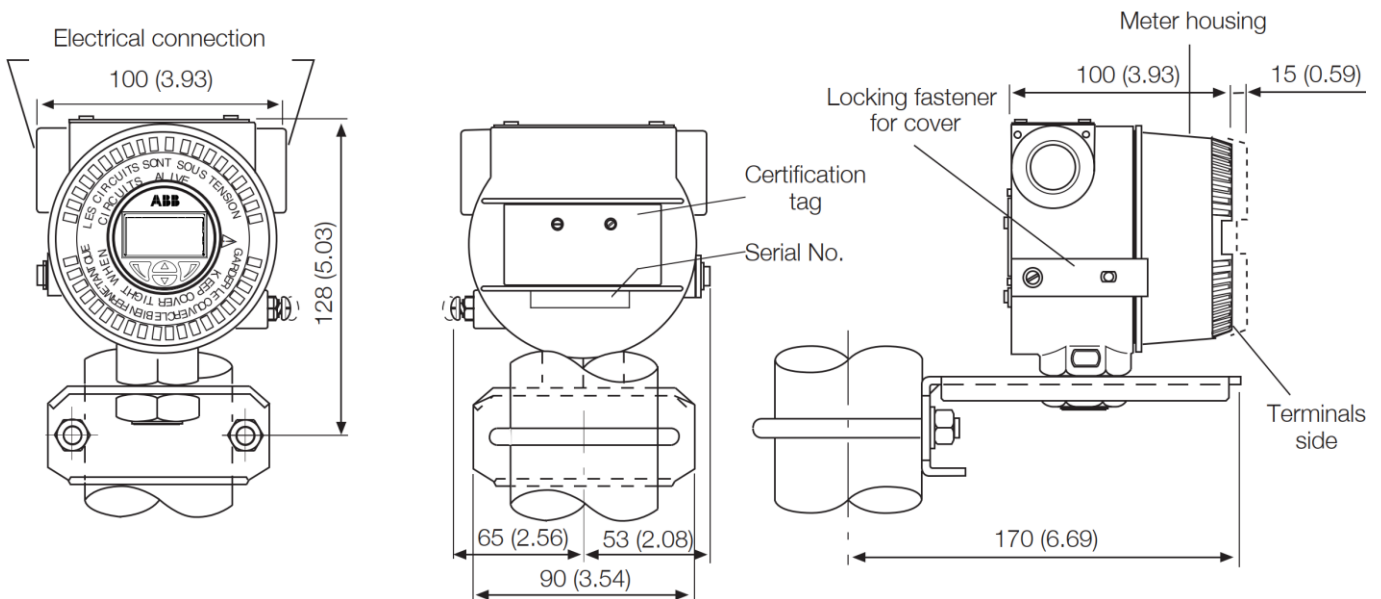
Figure 9: Field housing with TTH300 (option HG)
