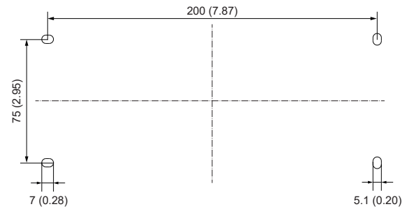
Fig. 25 Drilling pattern of stainless steel enclosure
