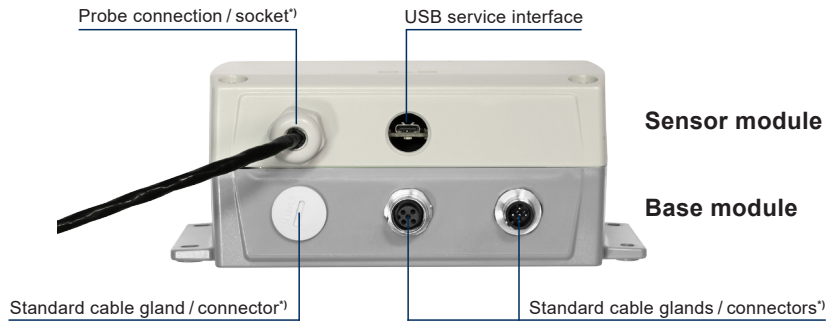
Fig. 2 hydroTRANS H50 connector-side view
