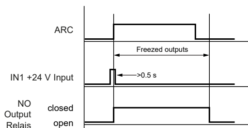
Fig. 15 ARC timing
