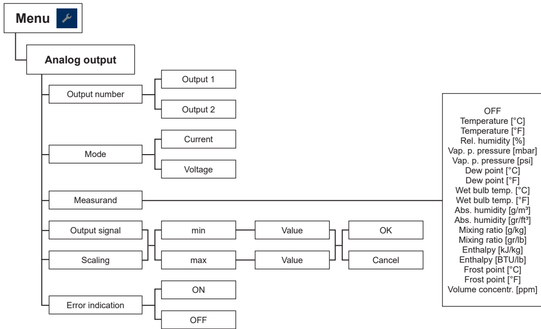
Fig. 47 Analogue output
