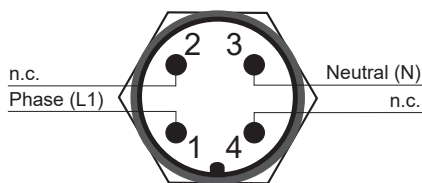
Fig. 36 Plug for power supply 100 - 240 V AC on polycarbonate enclosure, front view
