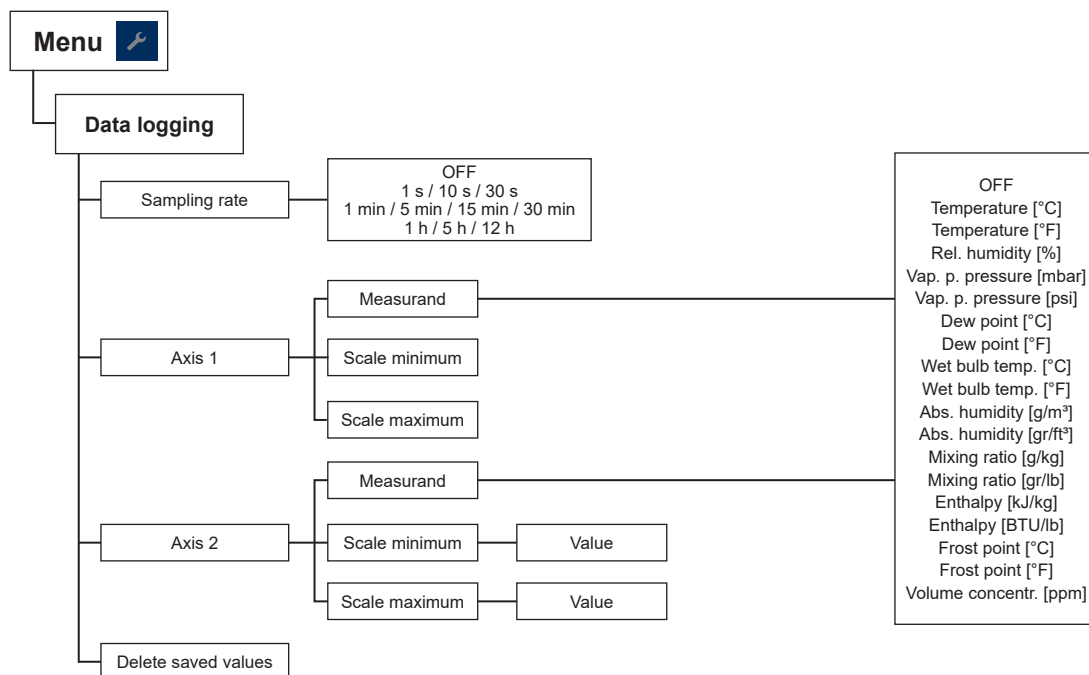
Fig. 45 Data logging
