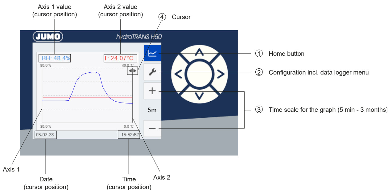
Fig. 11 Data logging
