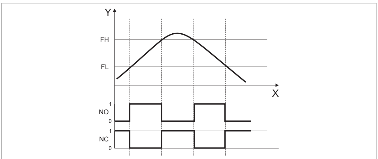
Function chart
