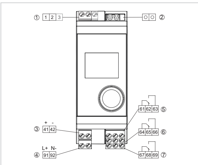
Wiring plan VEGAMET 141
