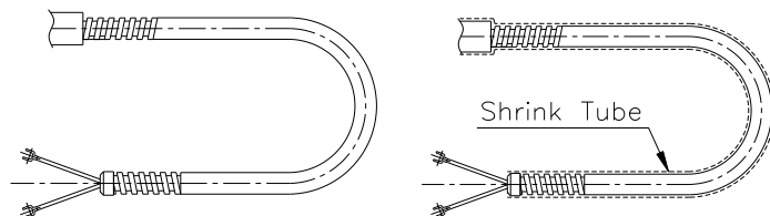
< Extended lead wire with steel armored tube type >
