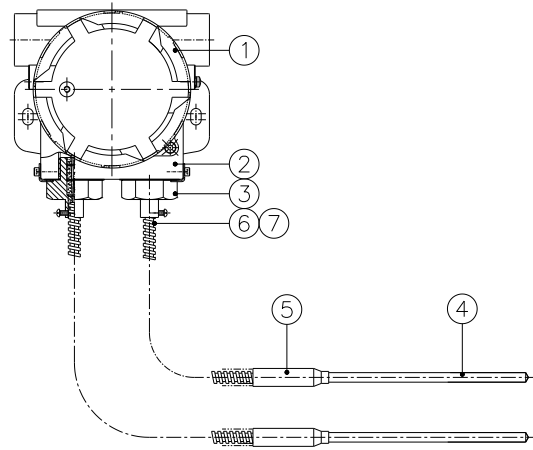
< Multi point head type >
