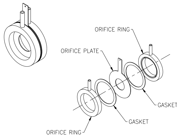
Orifice Plate & Ring
