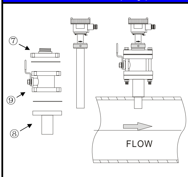
Install with Ball Valve (Flange)
