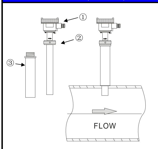
Direct Installation (Flange)
