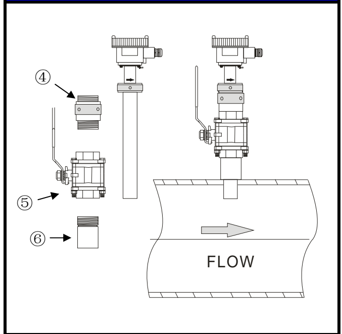
Install with Ball Valve (M60 Thread with Adapter)
