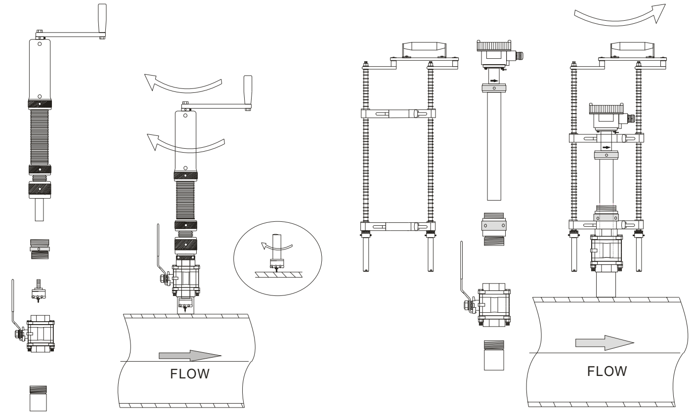
Hot-Tap Machine
