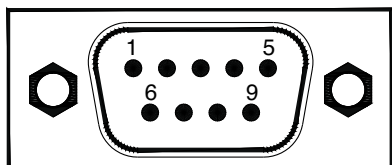
Figure 12 GF_VEDO HL RS-232 port connector
