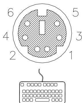
Figure 20 GF_VEDO HL PS2 port connector for Mouse and Keyboard
