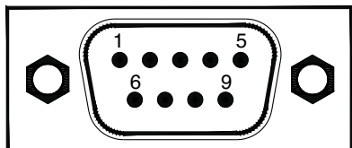
Figure11 RS-485 connector for GF_VEDO HL port
