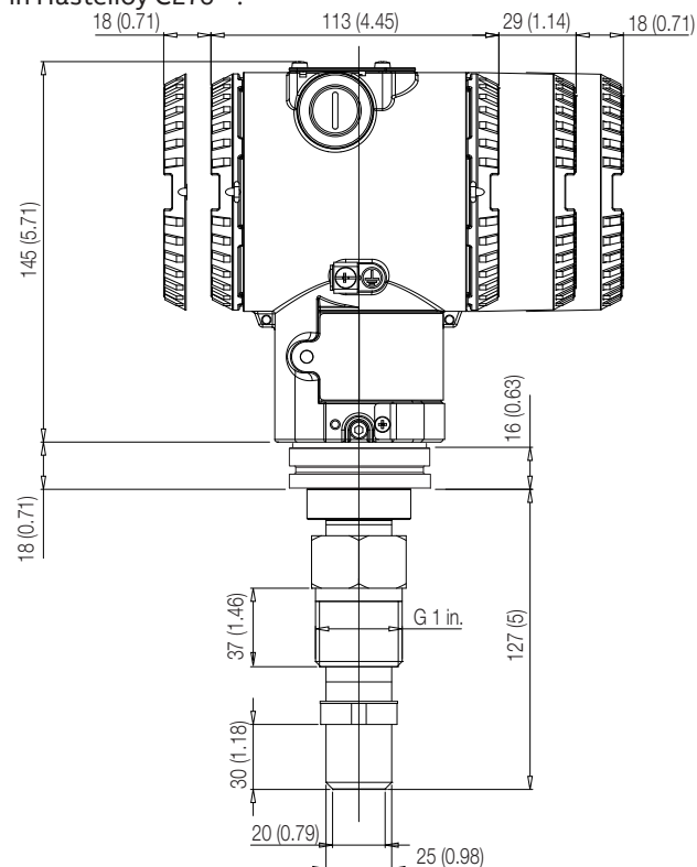
Figure 27: S26KN with ball valve connection
