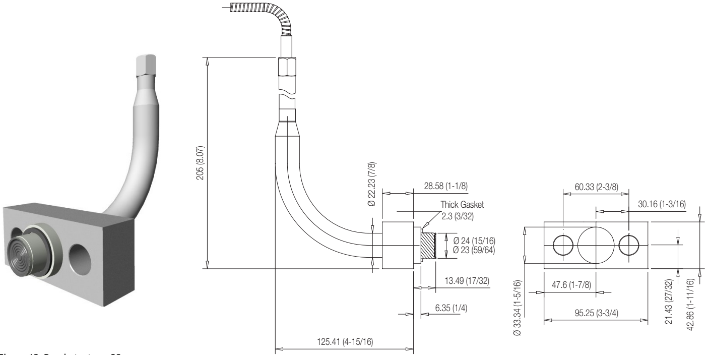
Figure 13: Bracket – type 89
