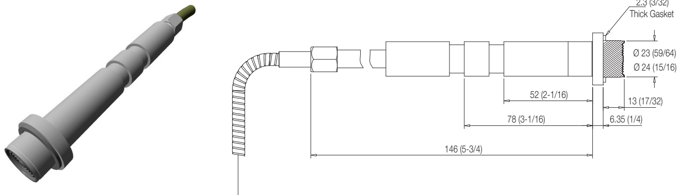
Figure 14: Universal – type 90
