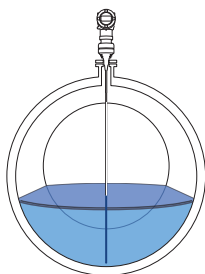
Horizontal cylinder
